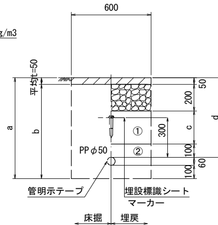
PPφ50
